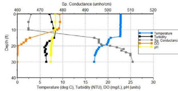
Figure 2. Field data taken at the dam site (2CBR20001; Figure 1) on 6/5/2017 at 08:00.
