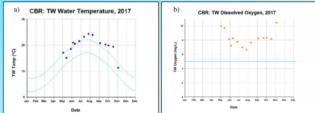
Figure 3. CBR time series data collected from the tailwater (2CBR10000; Figure 1): a) water temperature; and b) dissolved oxygen.
